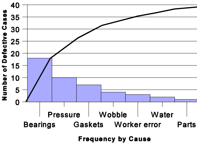
Figure 17-5. Pareto diagram.
