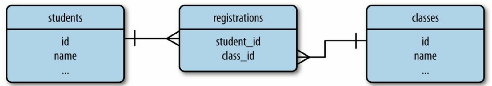
Figure 12-1. Many-to-many relationship example
