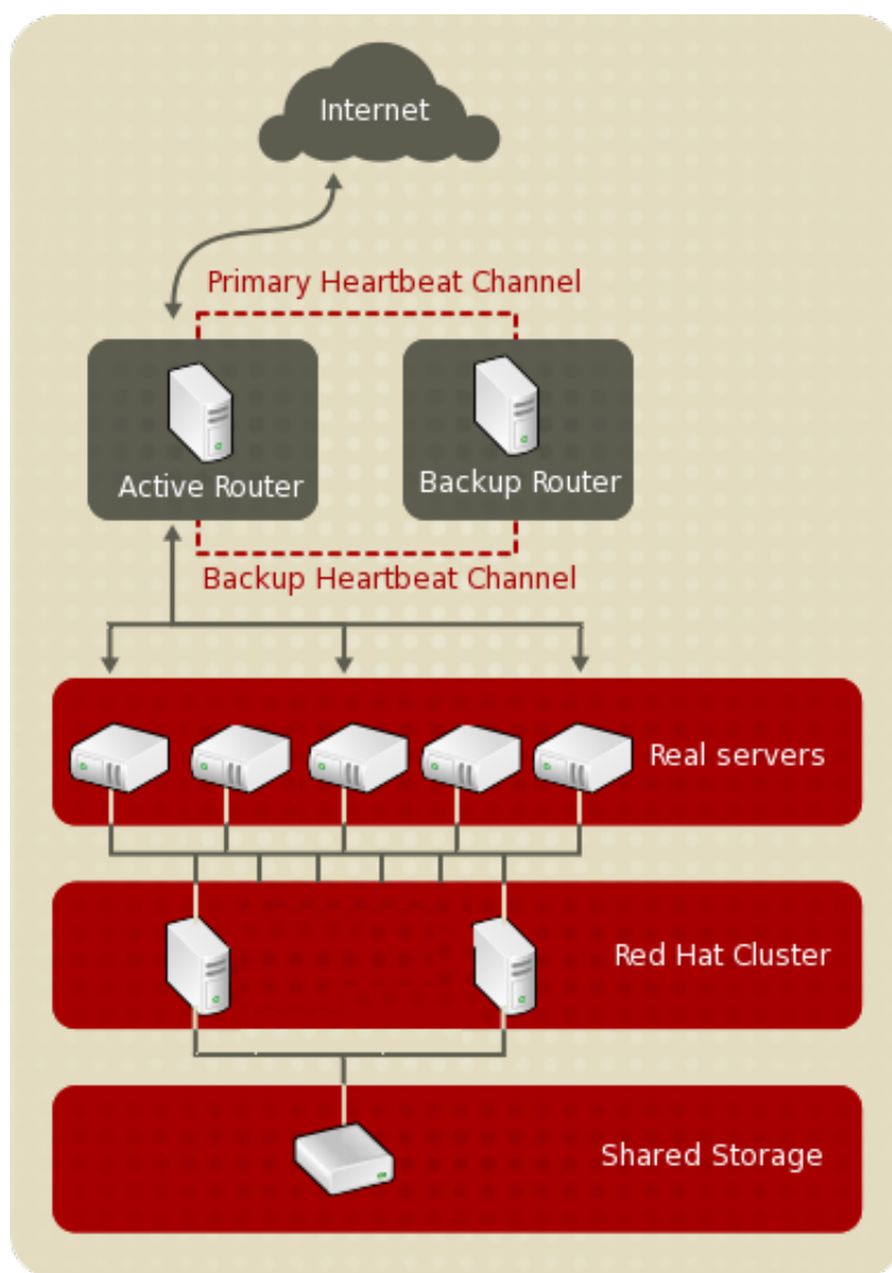
Figure 1.2. A Three-Tier Load Balancer Add-On Configuration
