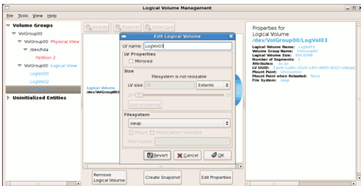
Figure 4.6. Edit Logical Volume
