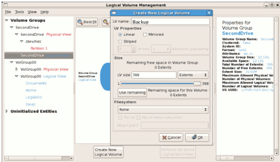
Figure 4.17. Create new logical volume
