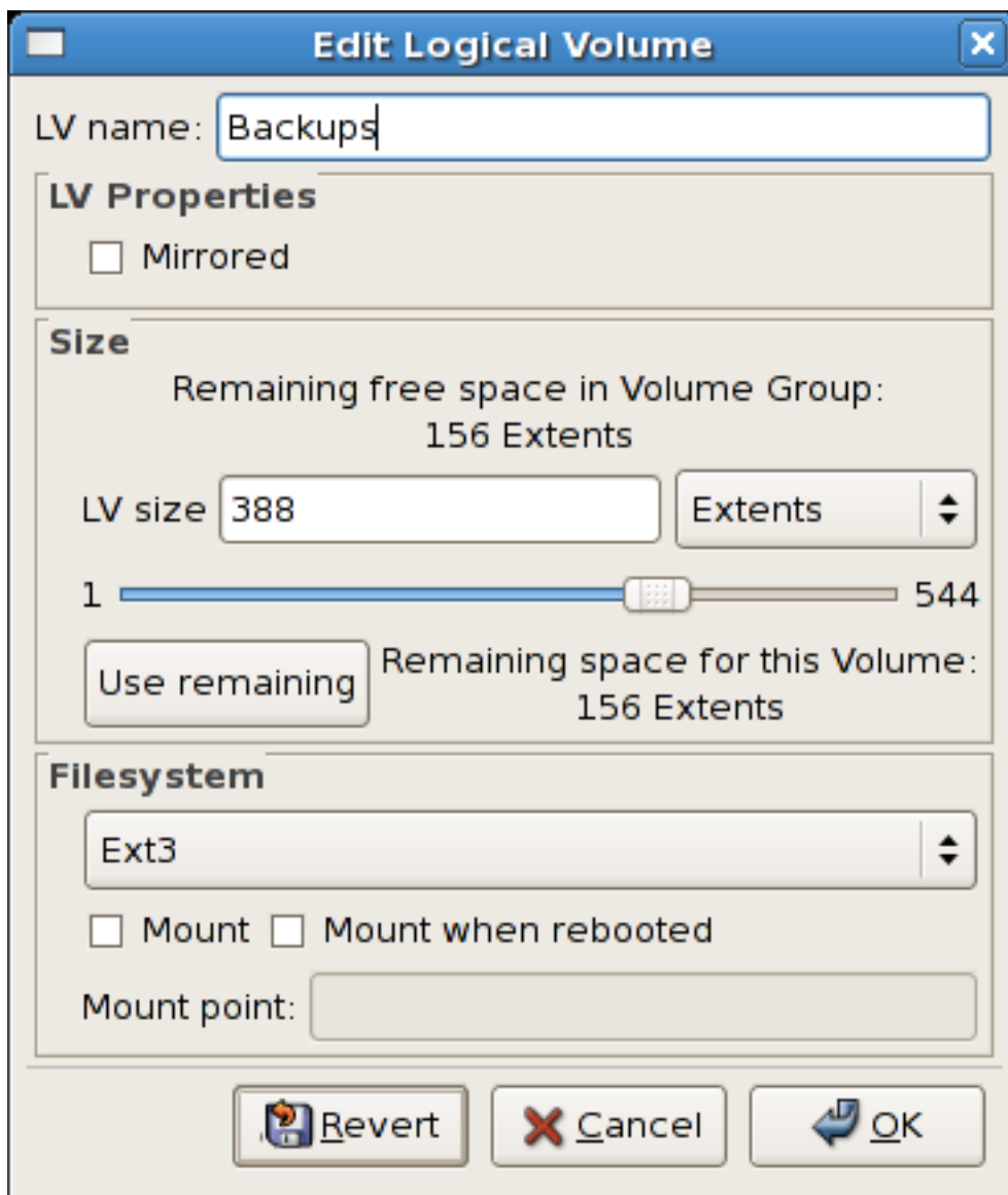
Figure 4.21. Edit logical volume
