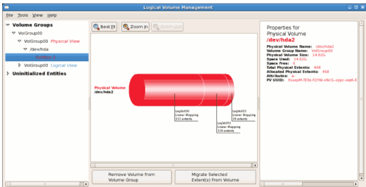
Figure 4.4. Physical View Window
