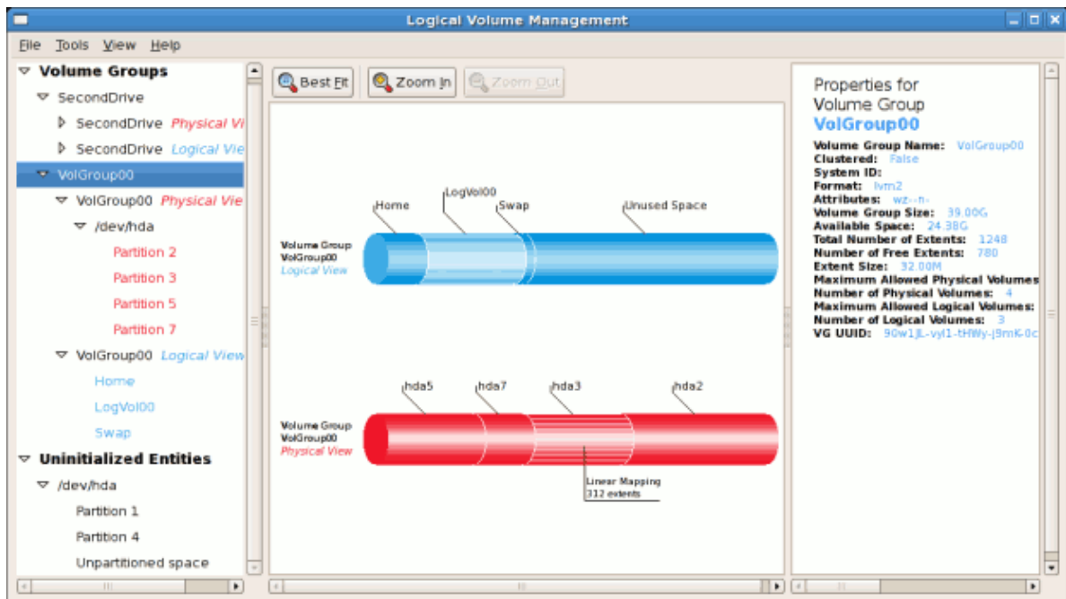
Figure 4.14. Logical and physical view of volume group
