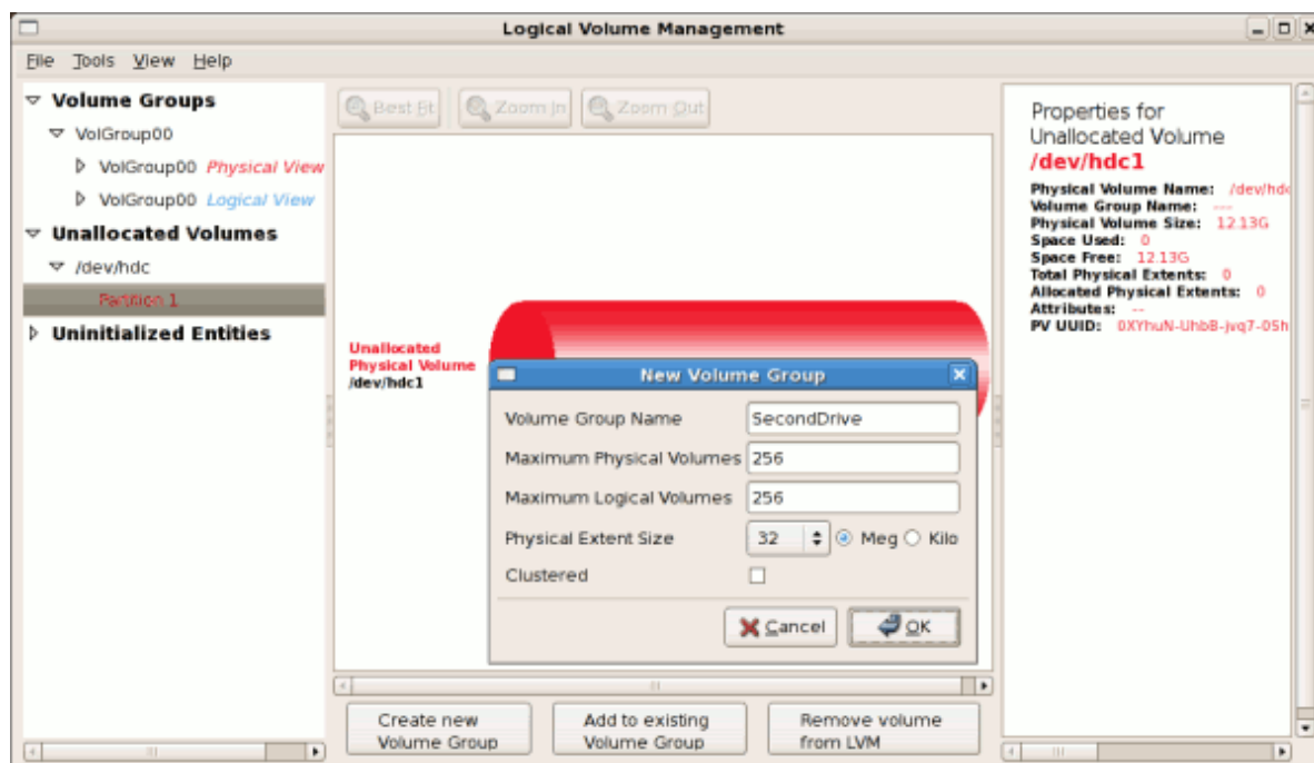
Figure 4.16. Create new volume group
