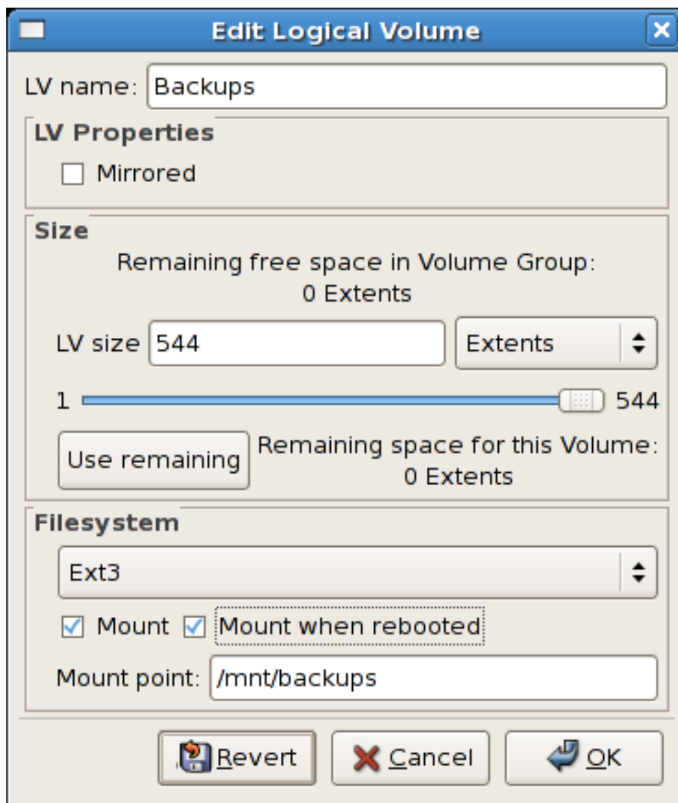
Figure 4.22. Edit logical volume - specifying mount options
