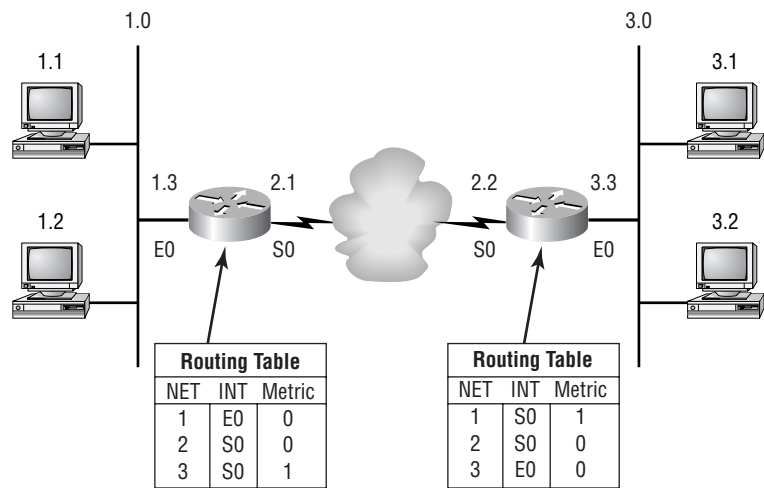
FIGURE 1.8 Routing table used in a router
