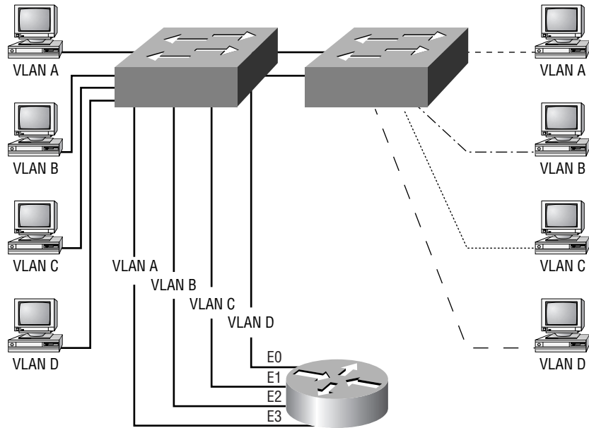
FIGURE 6.3 Switches removing the physical boundary
