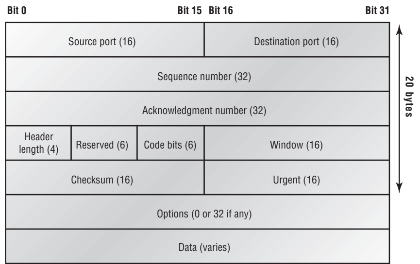
FIGURE 3.3 TCP segment format
