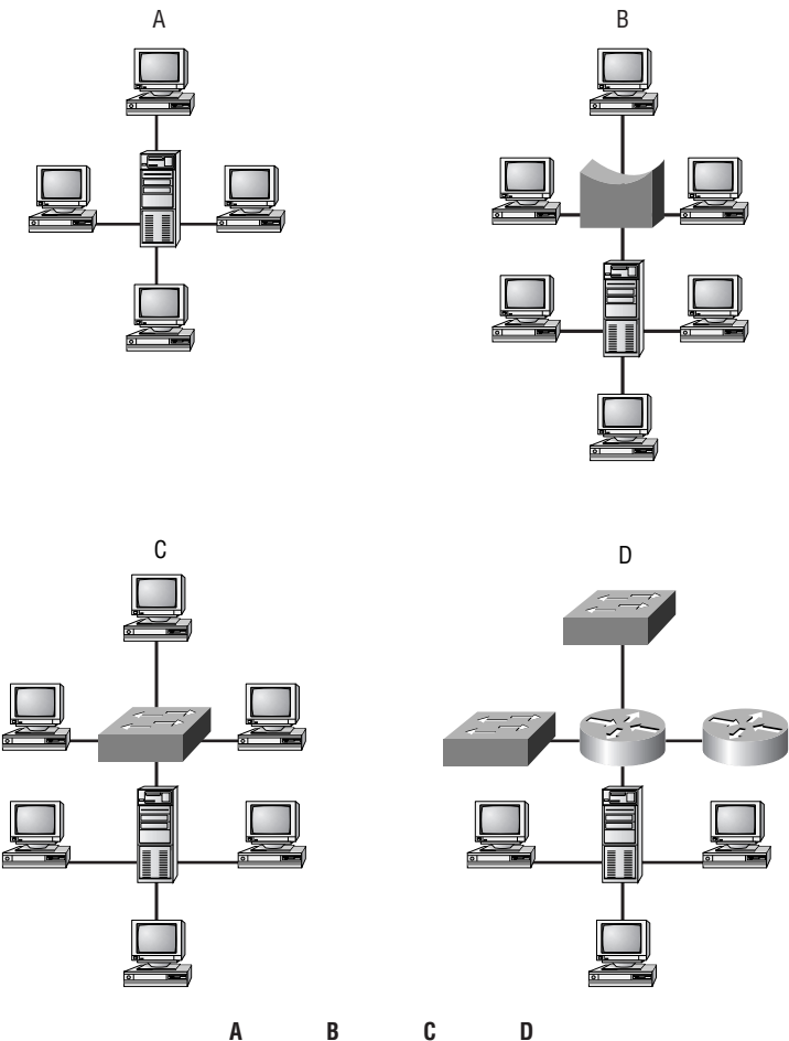
FIGURE 1.23 Identifying the amount of collision and broadcast domains
