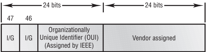
FIGURE 1.10 Ethernet addressing using MAC addresses
