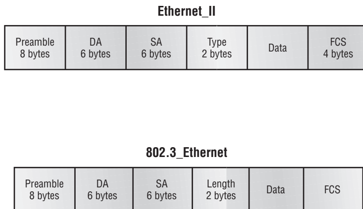
FIGURE 1.11 802.3 and Ethernet frame formats
