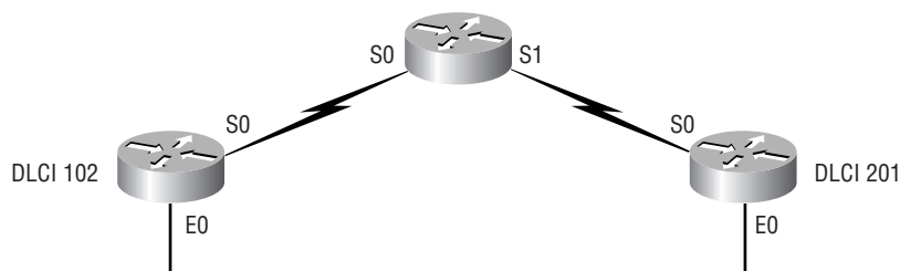
FIGURE 10.9 Frame Relay lab
