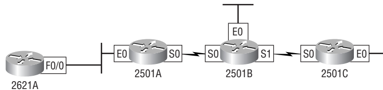
FIGURE 5.4 IP routing example 2 with more routers
