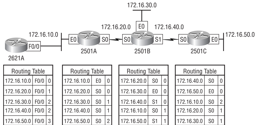
FIGURE 5.7 Converged routing tables
