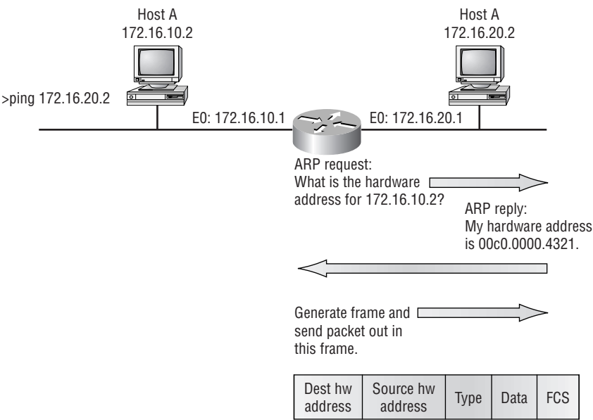
FIGURE 5.3 Frame generated from router
