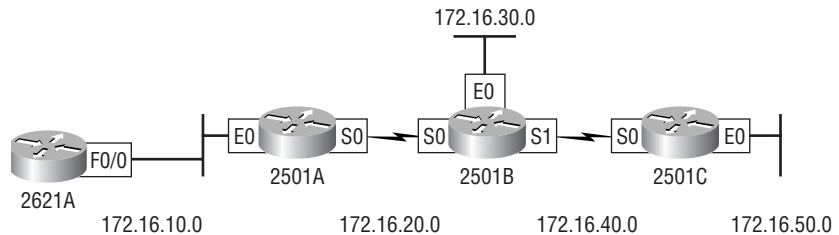
FIGURE 5.9 Hands-on lab internetwork
