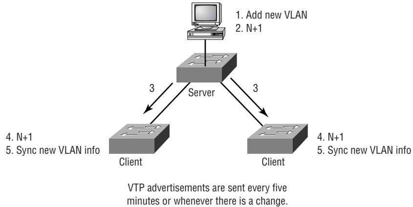
FIGURE 6.5 VTP revision number
