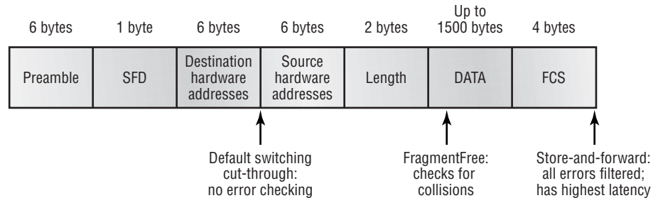
FIGURE 2.6 Different switching modes within a frame
