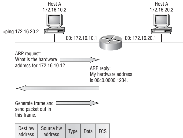
FIGURE 5.2 Frame generated from Host A
