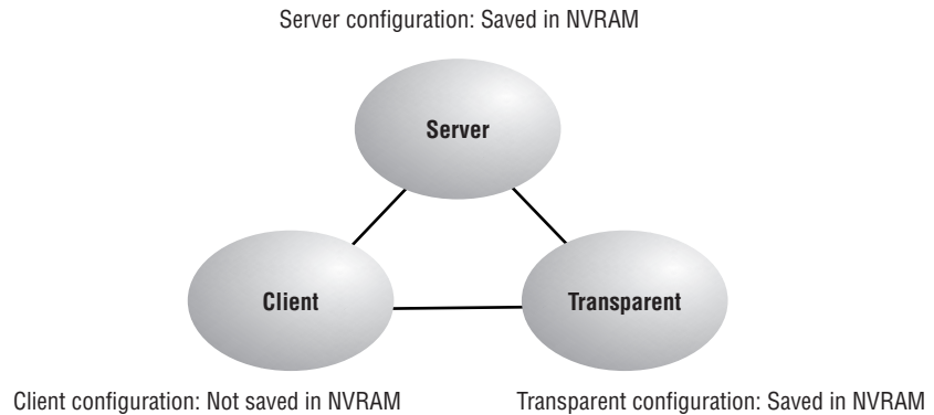
FIGURE 6.4 VTP modes
