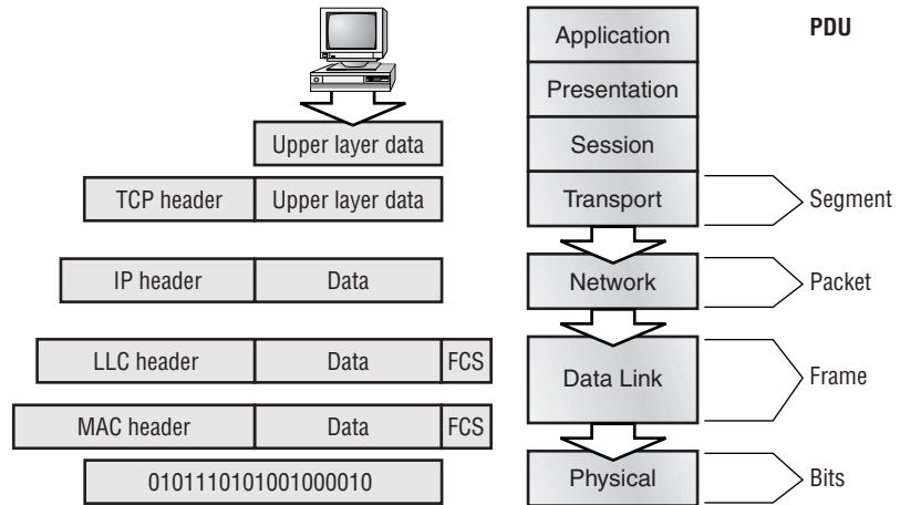
FIGURE 1.13 Data encapsulation
