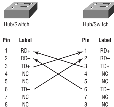
FIGURE 1.19 UTP crossover implementation
