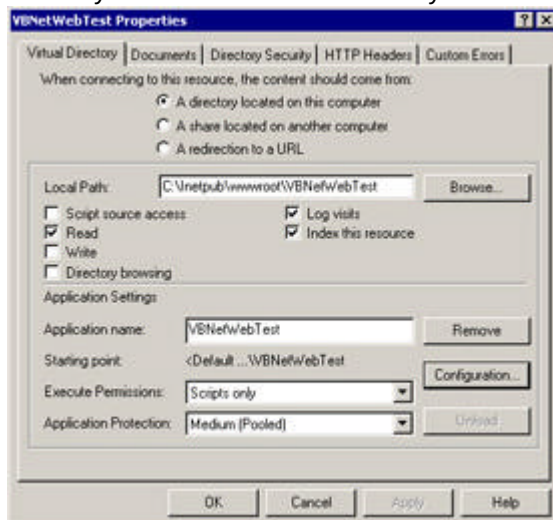
Figure 16.7: VBNetWebTest Properties dialog
