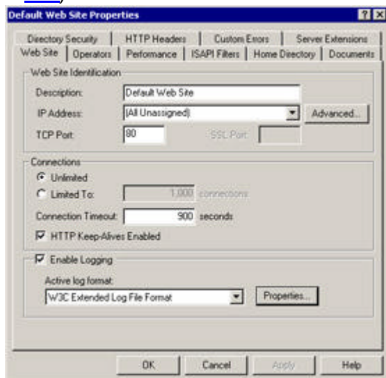
Figure 11.4: The IIS Default Web Site Properties dialog
