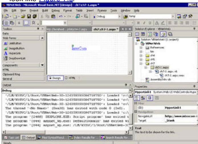
Figure 7.5: Visual Studio Web Form design surface after adding a HyperLink server control. Run the Web Form again. Did ASP.NET add the munged URL to the hyperlink? Move your cursor over it to see the link in the status bar. You'll see the hyperlink, but it hasn't been altered to contain the ASPSessionID. Of course, it wouldn't make any sense to add the ASPSessionID to an external link. You may be surprised by the fact that the SessionID shows up in the Response.Write.
