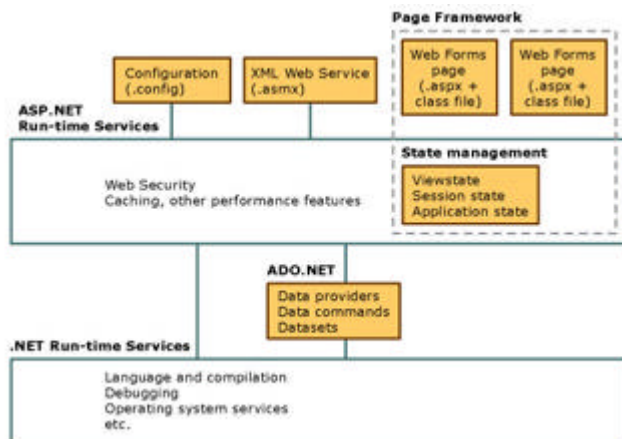
Figure 4.1: ASP.NET integration with the .NET framework
