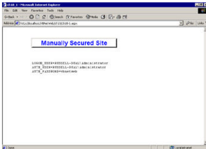
Figure 18.6: User entered vaild username/password combination
