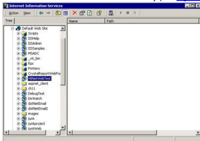
Figure 16.6: Internet Information Services applet after creating the VBNetWebTest virtual directory
