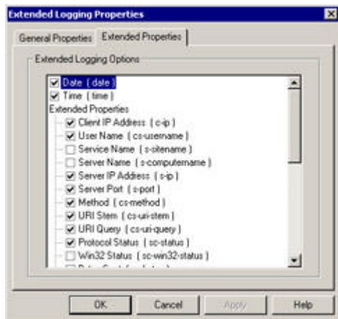
Figure 11.6: IIS Extended Logging Properties dialog for the W3C extended log format
