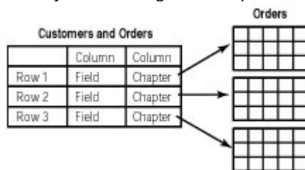
Figure 13.8: Shaped recordset where each customer record has a chapter column consisting of another recordset containing multiple orders for that customer
