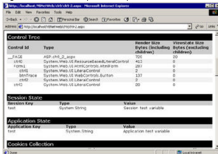
Figure 9.14: Trace output with explicit Trace.Write results (screen 2)
