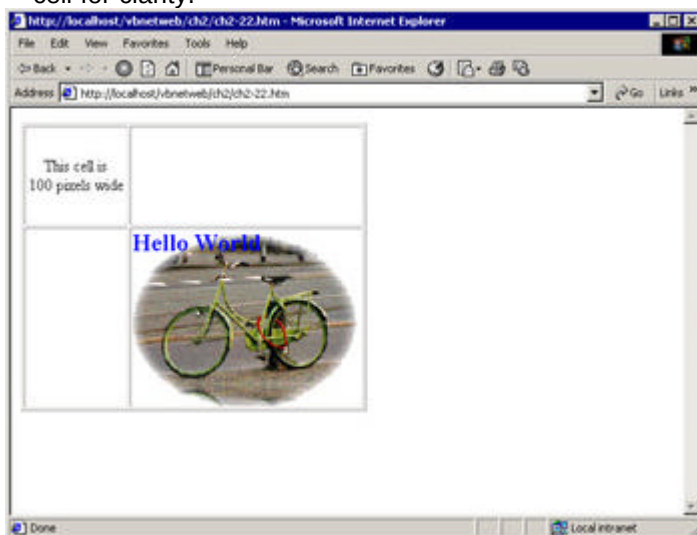
Figure 2.20: Controlling element position with tables (ch2-22 .htm)
