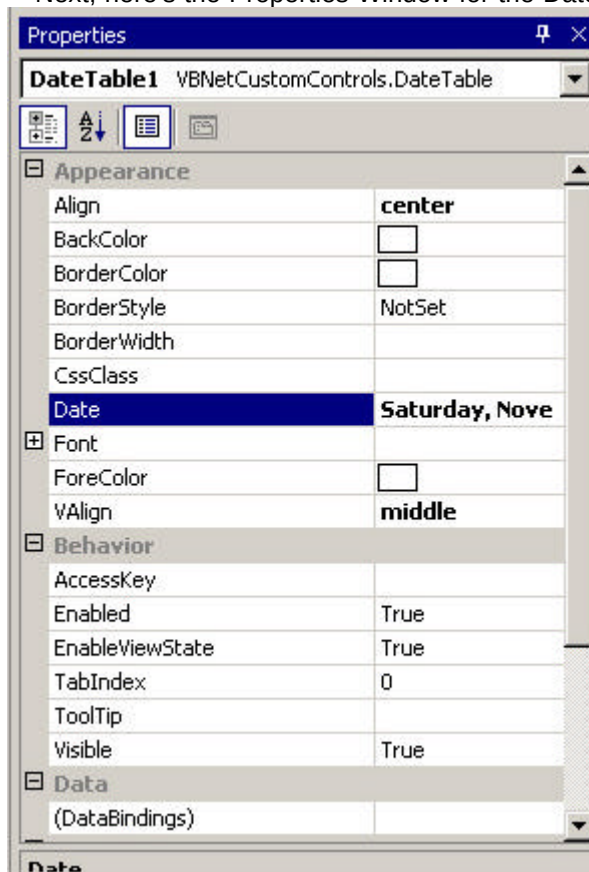
Figure 23.6: DataTable Custom Control Properties Window
