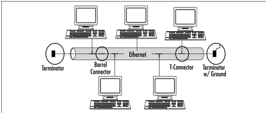
Figure 6.16 Sample Coax Segment
