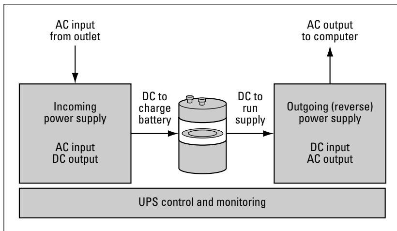
Figure 21-9: UPS schematic
