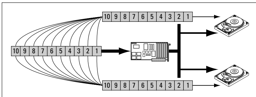
Figure 8-7: RAID 1 offers better reliability than RAID 0 or conventional disk setups, but does not increase performance.
