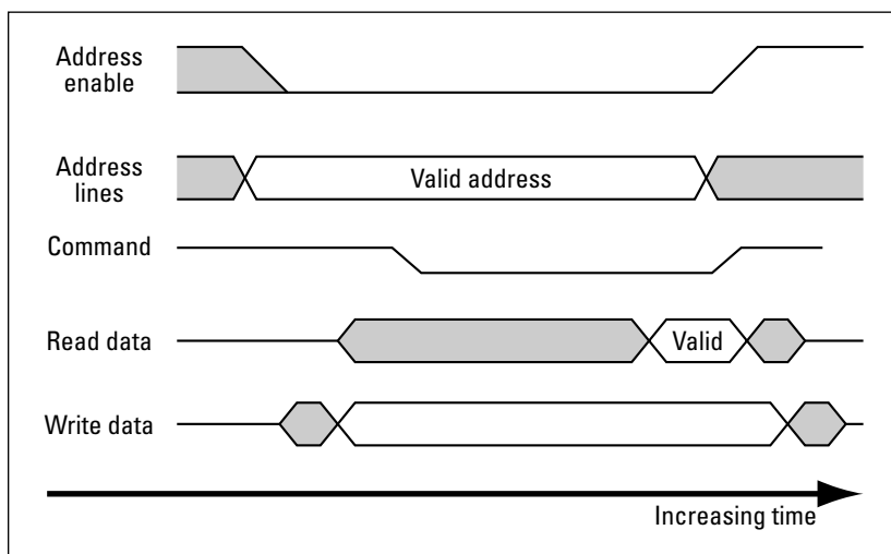
Figure 5-2: The operation of the ISA bus is defined by a simple set of signals and rules.
