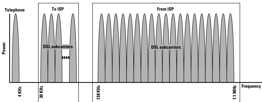
Figure 11-2: DSL spectrum occupancy
